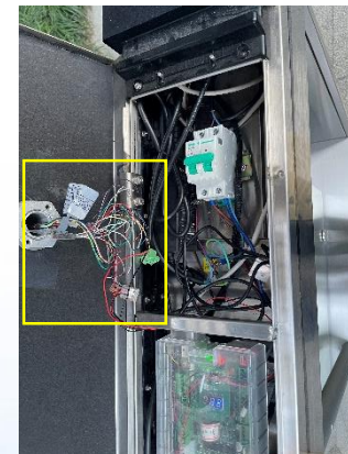
3. For turnstiles with standalones – wiring the cables through the installation bracket
